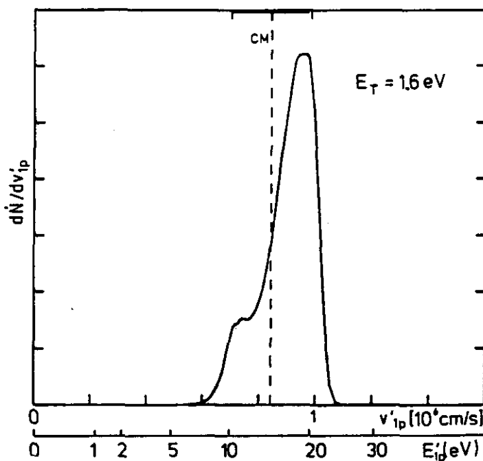
Figure 71. Product velocity distribution d\dot{N}/dv'_{ip} for the charge-transfer reaction \text{Ar}^{2+} + \text{He} \rightarrow \text{Ar}^{+} + \text{He}^{+} measured at a collision energy of 1.6 eV in the guided-ion-beam apparatus. The upper scale marks the position of the center-of-mass velocity and the range of the Newton circle. It is evident that at this energy forward scattering prevails.
