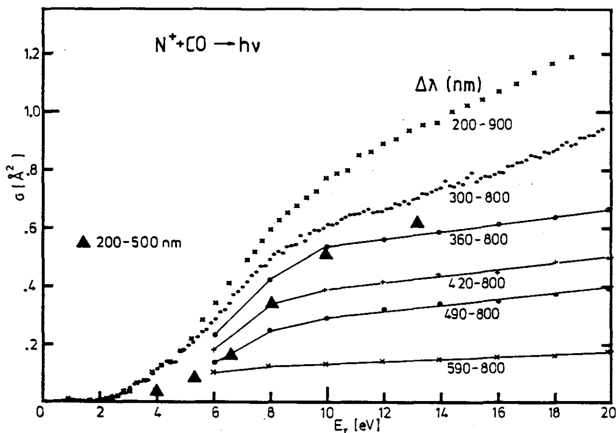
Figure 77. Integral cross sections for formation of luminescent products ( \text{CO}^+ , \text{CN}^+ , etc.) in \text{N}^+ + \text{CO} collisions recorded for selected wavelength ranges using the apparatus shown in Fig. 46. The triangles are from Neuschäfer et al. (1981).
