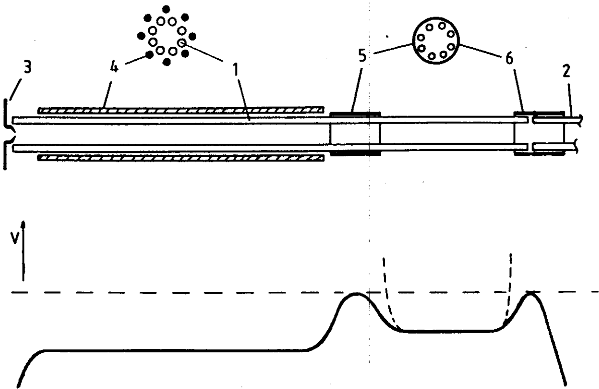
Figure 30. System of two octopoles (1,2) with electrodes for ion injection (3) and for field correction (4–6). Correction electrode (4) consists of eight rods, staggered as indicated, (5) and (6) are cylinders. The lower panel shows a schematic representation of the dc potential along the axis of the system. In this example, the electrode (4) was used to lower the potential slightly, while (5) and (6) were used to create barriers.
