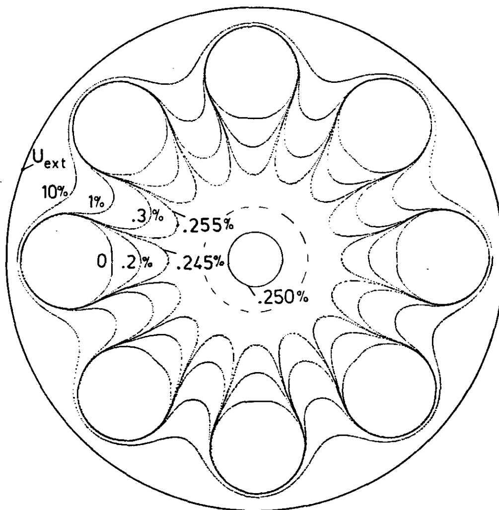
Figure 17. Contour plot of the electrostatic potential inside an octopole caused by a voltage U_{\text{ext}} applied to the surrounding cylinder. The potential of the eight rods is set to zero. The height of the equipotential lines is given relative to the external voltage. For the geometry shown, the potential on the centerline is shifted by 0.25%.
