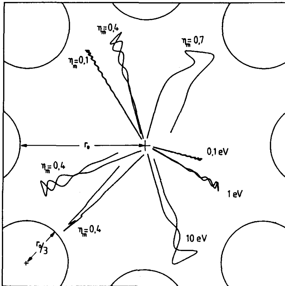
Figure 11. Characteristic ion trajectories in an octopole illustrating different operating conditions. All ion trajectories start in the center of the octopole. The examples with \eta_m = 0.1 , 0.4 , and 0.7 illustrate that with increasing \eta the amplitude of the wiggling motion increases and that the number of oscillations during one reflection from the rf wall decreases. For the three energies ( 0.1 , 1 , and 10 \text{ eV} ) the values \varepsilon and V_0 are constant. In the remaining trajectories ( \eta_m = 0.4 ) only the starting angle has been changed. In one case, the small oscillations \mathbf{R}_1(t) are parallel to the secular motion \mathbf{R}_0(t) ; in the other, they are orthogonal.
