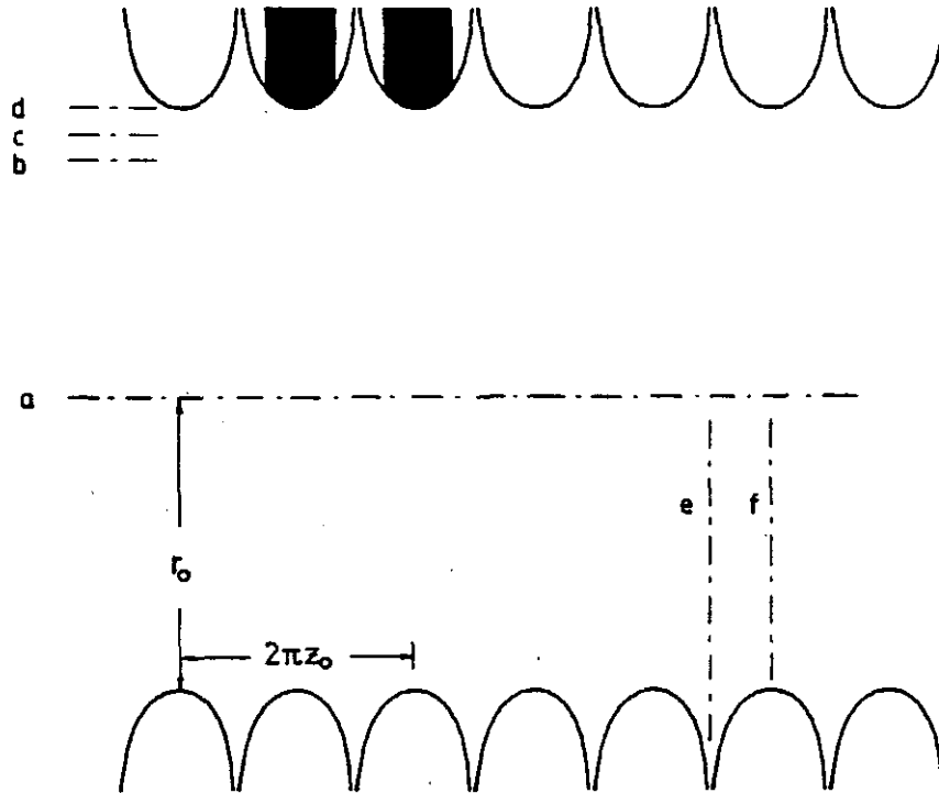
Figure 7. Equipotential lines of a rotationally symmetric ring electrode trap, defined in Eq. (34). The actual shape of the electrodes is marked in black (see Section III E). The letters a – f indicate locations along which Fig. 8 shows cuts through the effective potential.
