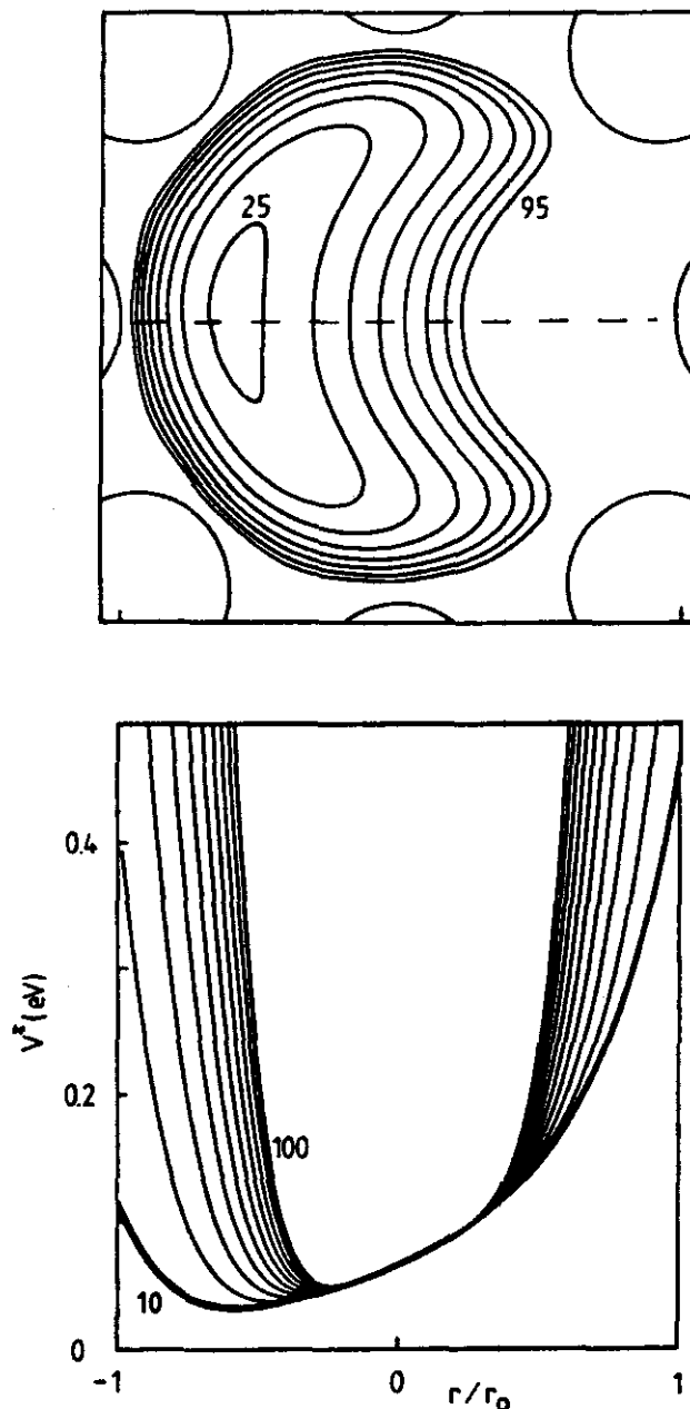
Figure 16. Influence of an electrostatic potential distortion. In this example one rod on the right is charged to +0.5 V. The upper panel shows a contour plot of the effective potential (in meV, 10-meV steps) for a low rf amplitude of 10 V. The lower panel is a cut through the potential along the dashed line and illustrates the influence of the rf amplitude as it is increased in 10-V steps.
