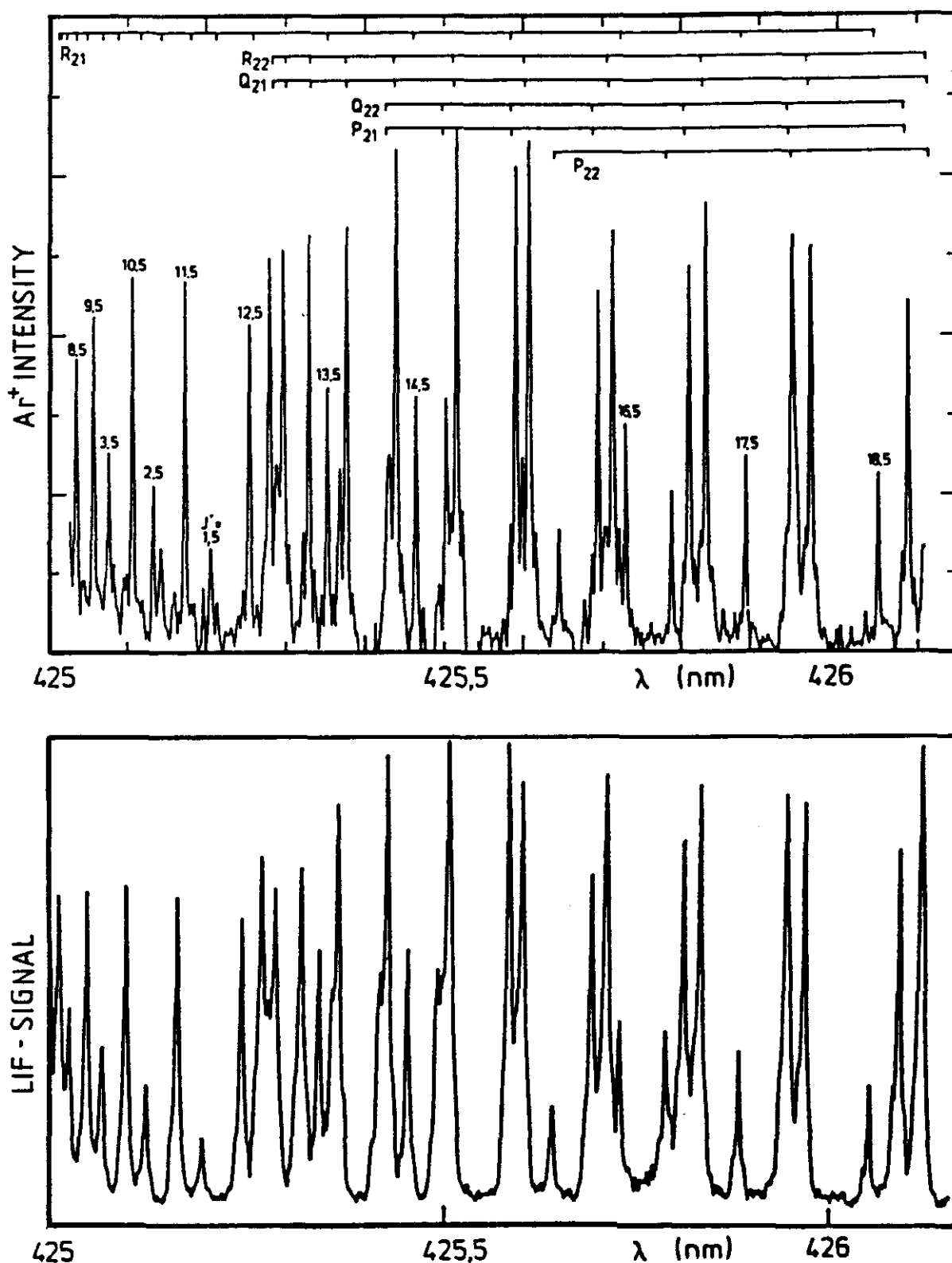
Figure 81. Laser excitation of \text{CO}^+ ions in an octopole. In both experiments the \text{CO}^+ ions were formed by electron bombardment in the rf storage ion source of the guided-ion-beam apparatus. The upper panel shows the wavelength dependence of \text{Ar}^+ charge-transfer products formed in low-energy collisions between laser excited \text{CO}^+(A^2\Pi) and Ar in the scattering cell. The lower panel depicts, in the same wavelength range, the laser-induced fluorescence signal from \text{CO}^+ ions trapped in the scattering cell between two potential barriers.
