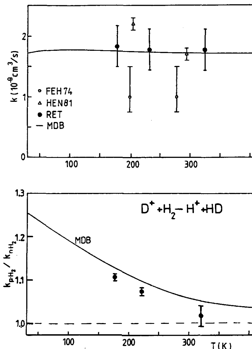
Figure 65. Thermal rate coefficients for \text{D}^+ + \text{H}_2 \rightarrow \text{H}^+ + \text{HD} . The upper panel shows a comparison of our ring electrode trap results ( \bullet ) with those from a flowing afterglow ( \circ ) (Fehsenfeld et al., 1974) and a SIFT ( \Delta ) (Henchman et al., 1981) apparatus. The solid line was determined using the statistical MDB theory (Gerlich, 1982). In all these experiments, normal- \text{H}_2 was used. The lower panel compares results obtained for 75% enriched para- \text{H}_2 and normal- \text{H}_2 . The reaction rate with \text{H}_2(j=0) increases with falling temperature due to the influence of the charge-quadrupole interaction, in reasonable accord with the statistical MDB theory.
