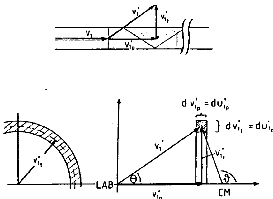
Figure 48. Scattering in an octopole. The upper part illustrates schematically the parallel and the transverse components of the product velocity vector \mathbf{v}_i' = (v_{i'p}, v_{i't}) . The lower part shows the cylindrical ring volume element in the velocity space, needed to define the doubly differential cross section d^2\sigma/du_{i'p}du_{i't} . In the figure on the right, \theta and \vartheta are the laboratory and center-of-mass scattering angles, respectively.
