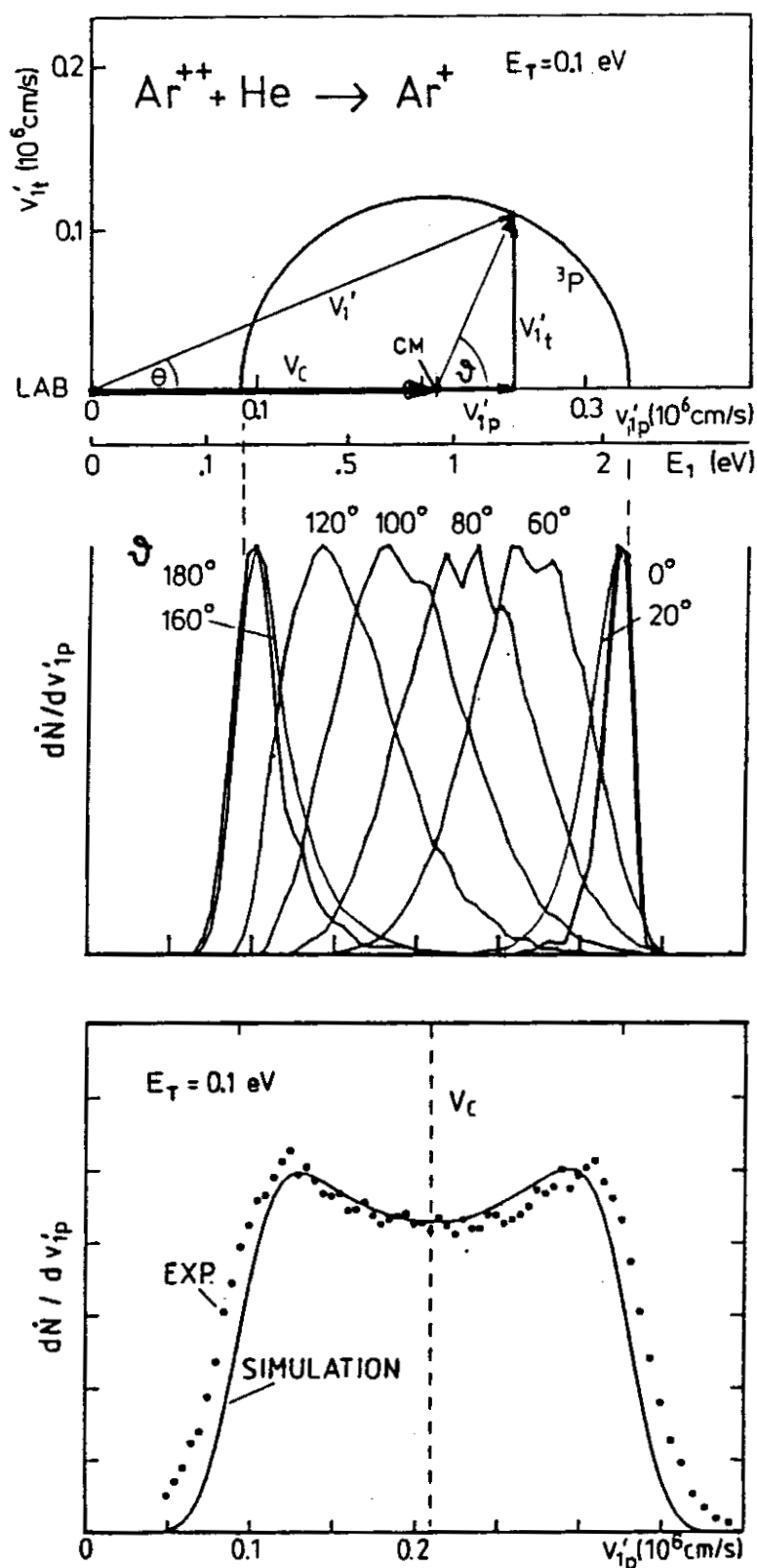
Figure 68. Differential scattering in the state-to-state charge-transfer reaction \text{Ar}^{2+} + \text{He} \rightarrow \text{Ar}^+ + \text{He}^+ in the guided-ion-beam apparatus. The upper panel depicts a nominal Newton diagram scaled for a collision energy of 0.1 eV. CM marks the origin of the center-of-mass system; the He target is assumed to be at rest. The laboratory and center-of-mass scattering angles are \theta and \vartheta , respectively. The projection of the final velocity v_1' onto the octopole axis, that is, the component v_{1p}' , is measured by time of flight. The product velocity distributions are broadened by the target motion, as illustrated in the middle panel. The lowest panel compares a measured velocity distribution with a simulation based on a weighted superposition of functions shown in the middle panel.
