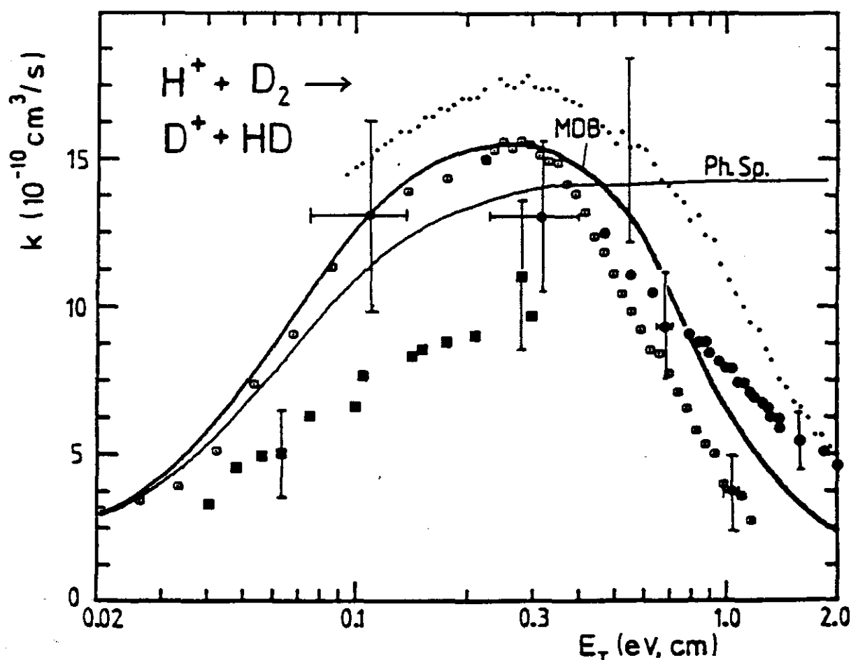
Figure 66. Energy dependence of the effective rate coefficient for the 46 meV endothermic proton-deuteron exchange \text{H}^+ + \text{D}_2 \rightarrow \text{D}^+ + \text{HD} measured with different techniques [merged beam \circ , guided ion beam \bullet (Ochs and Teloy, 1974), and \bullet (Müller, 1983), DRIFT \blacksquare (Villinger et al., 1982)]. The heavy line is the result from the statistical MBD theory (Gerlich, 1982), and the thinner line is the prediction based on conventional phase space theory.
