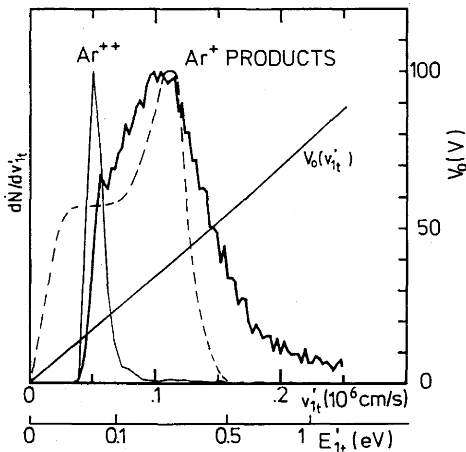
Figure 69. \text{Ar}^+ transverse product velocity distribution d\dot{N}/dv'_{1t} (heavy line) for the state-to-state charge-transfer reaction \text{Ar}^{2+} + \text{He} \rightarrow \text{Ar}^+ + \text{He}^+ , obtained by variation of the rf guiding field. The dashed line shows a simulation that only accounts for the thermal broadening. Deviations from the experimental \text{Ar}^+ curve are explained in the text. The maximum of the product distribution is situated slightly above v'_{1t} = 1 \times 10^5 cm/s in accordance with the Newton diagram in Fig. 68. The narrow \text{Ar}^{2+} distribution has been determined by differentiating the rf-dependent transmission function of the primary beam. The slightly curved line shows the relation between the maximum guided transverse velocity and the amplitude V_0 , as obtained from Eq. (84).
