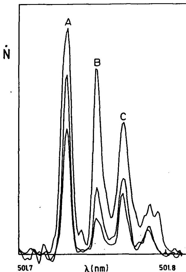
Figure 51. Laser fragmentation spectrum of O_2^+ for three laser energies. The spectra were recorded at pulse energies of 0.1 mJ, 0.2 mJ, and 1.7 mJ. Note that line A is strongly saturated. The energy necessary to reach 63.2% fragmentation is different for each of the depicted transitions, 0.13 mJ for A, 0.52 mJ for B, and 0.21 mJ for C.
