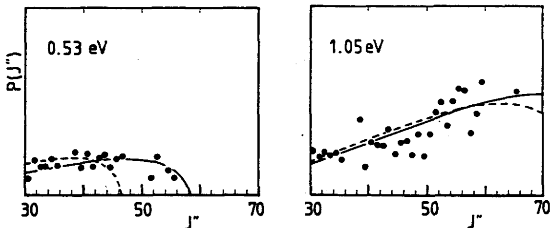
Figure 84. Relative populations of rotational levels for \text{O}_2^+(a^4\Pi_u, v=0) product ions formed in \text{Ar}^+ + \text{O}_2 collisions at 0.53 eV and 1.05 eV. The depicted probabilities were extracted from photofragmentation spectra [see, for example, Fig. 83 and Scherbarth and Gerlich (1989)]. The lines are the microcanonical equilibrium distributions for the two \text{Ar}^+(^2P_1) states.
