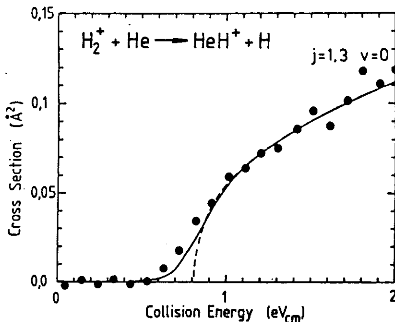
Figure 80. Integral cross section of the endothermic reaction \text{H}_2^+(v=0) + \text{He} \rightarrow \text{HeH}^+ + \text{H} in the threshold region. State-selective preparation of \text{H}_2^+ ions was achieved by multiphoton ionization using the quadrupole photoionization source in the guided-ion-beam apparatus. The data points are in reasonable agreement with the effective cross section (heavy line) calculated from an assumed threshold onset (dashed line) [Eq. (91)].
