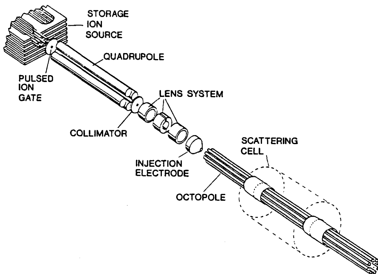
Figure 45. Perspective view of the major elements of a typical guided-ion-beam apparatus. Ions are created in a storage ion source, are mass and energy selected in a quadrupole and are injected into an octopole via a funnellike electrode. The scattering cell usually consists of a gas-containing cylinder surrounding the octopole. The ion beam is pulsed by opening the gate at the exit of the ion source and by pulsing the two halves of the middle element of the lens system.
