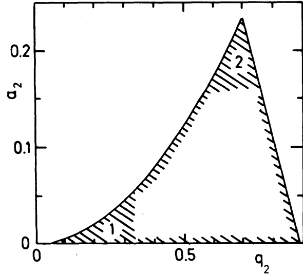
Figure 24. Lowest zone of stability of the Mathieu ( a_2, q_2 ) diagram. The boundary lines are given by a_2 = \frac{1}{2}q_2^2 - \frac{7}{128}q_2^4 \dots and by a_2 = 1 - q_2 - \frac{1}{8}q_2^2 \dots (Dawson, 1976). Region 2 is used for high-resolution mass filter operation. In region 1 the adiabatic approximation is valid.
