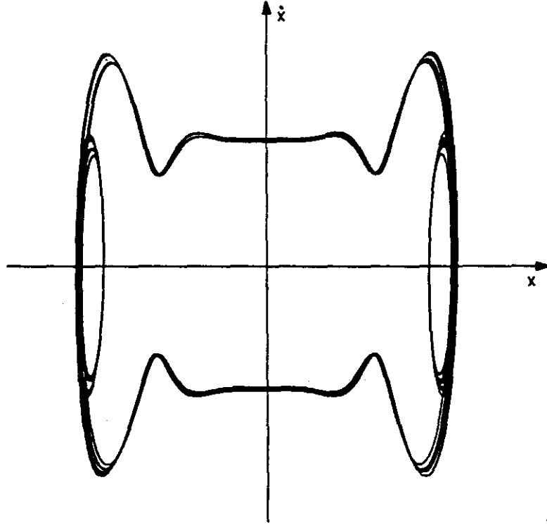
Figure 5. Phase space (x, \dot{x}) representation of a stable one-dimensional trajectory started with \eta_c = 0.65 in the vicinity of the periodic orbit \Omega/\omega = 10 ( \eta_c = 0.6454\dots ).
