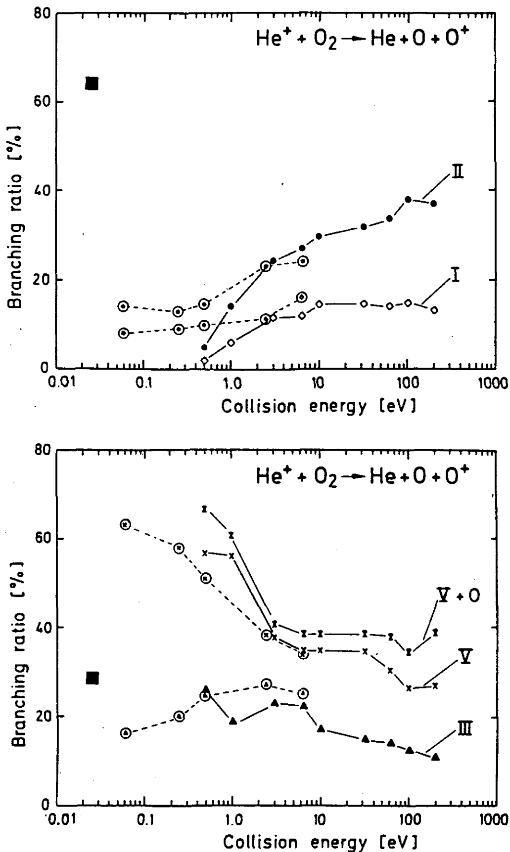
Figure 74. Branching ratios of the different \text{O} + \text{O}^+ channels (I–V) populated in dissociative charge-transfer collisions of \text{He}^+ with \text{O}_2 . The data at high energies, connected with solid lines, were obtained with a differential scattering apparatus (Bischof and Linder, 1986). The two squares are near-thermal results, derived from an ICR trap experiment, combining channels (I + II) and (III + V) (Mauclaire et al., 1979). The guided-ion-beam results, connected with dashed lines, close the energy gap between thermal energies and those accessible in standard beam techniques.
