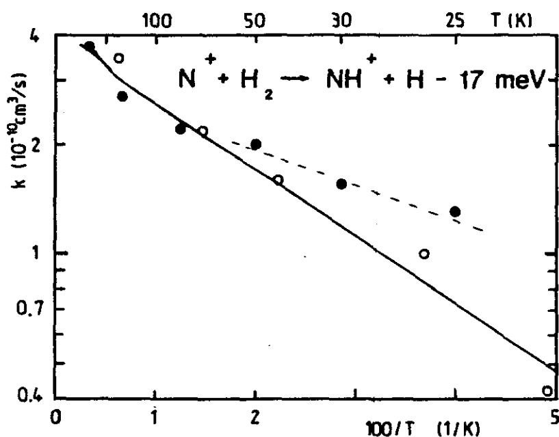
Figure 43. Arrhenius plot of the temperature dependence of the rate coefficient for the endothermic ion-molecule reaction N^+ + H_2 \rightarrow NH^+ + H . The phase-space calculation (Gerlich, 1989b) (solid line) has been adjusted to the CRESU results (Marguette et al., 1988) (○) by using \Delta H^0 = 17 meV. Possible explanations for the slight deviations from our trap measurements (●) are given in the text.
