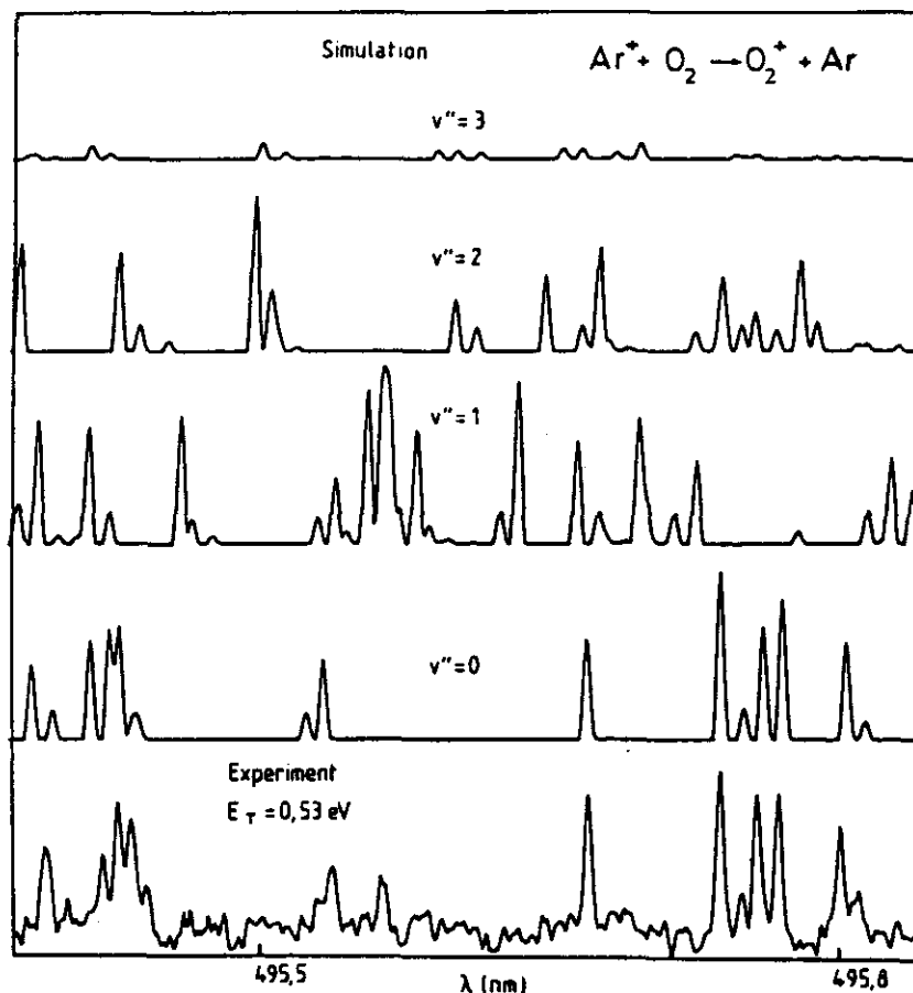
Figure 83. Laser-induced fragmentation of \text{O}_2^+ products recorded using the guided-ion-beam apparatus shown in Fig. 46. The lowest panel shows a small section of the experimental \Delta v = 3 photofragment spectrum of \text{O}_2^+(a^4\Pi_u) products populated in the \text{Ar}^+ + \text{O}_2 charge-transfer reaction. The upper curves are simulated spectra calculated separately for the accessible product vibrational states v'' = 0-3 . For the rovibrational states a statistical population was assumed.
