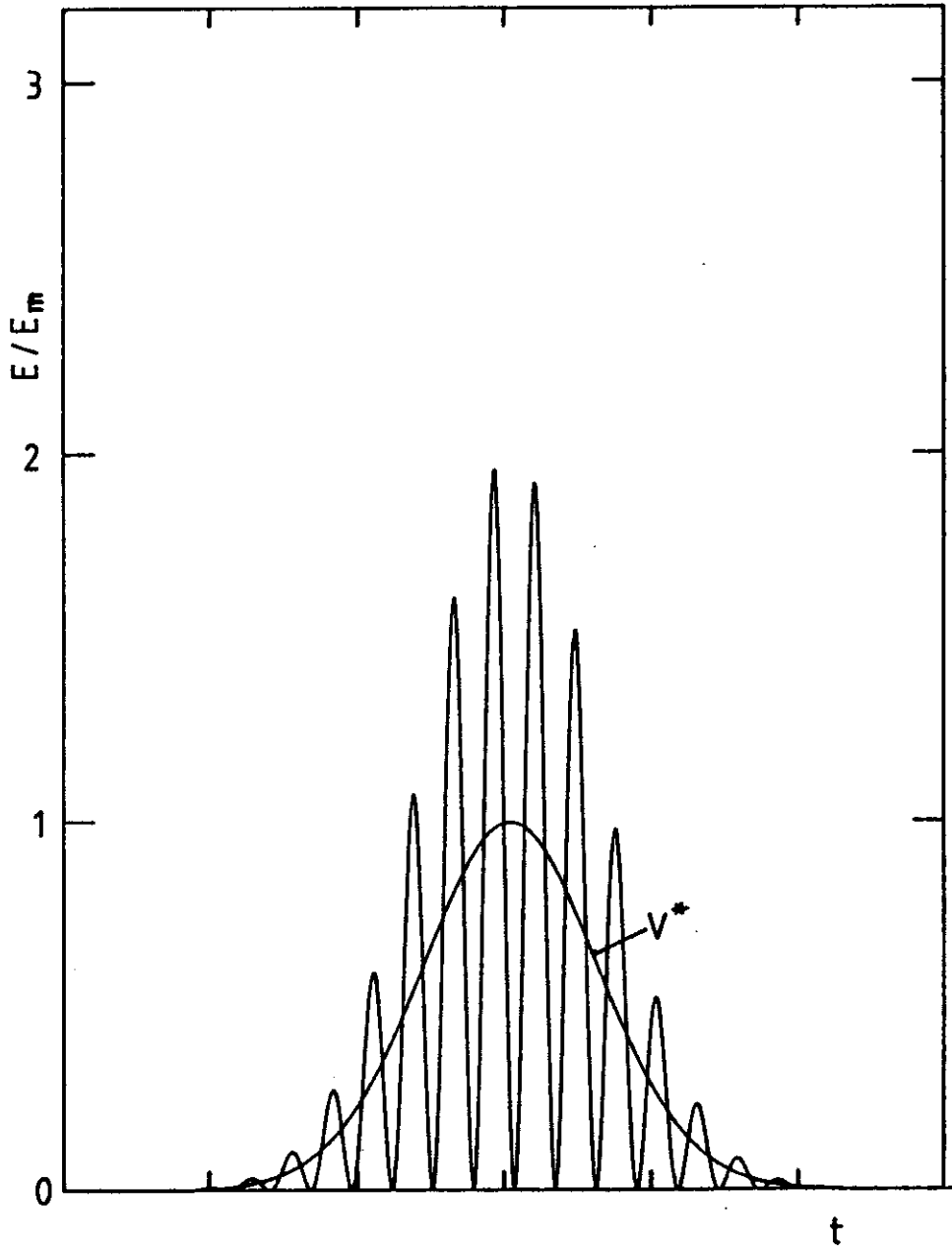
Figure 18. Time dependence of the kinetic energy ( \frac{1}{2}m\dot{\mathbf{R}}_1^2 ) and of the effective potential energy V^* during one reflection from an rf wall. The oscillatory line represents the kinetic energy of the wiggling motion, which varies between 0 and 2E_m . The smooth line shows the increase of the effective potential energy along \mathbf{R}_0(t) .
