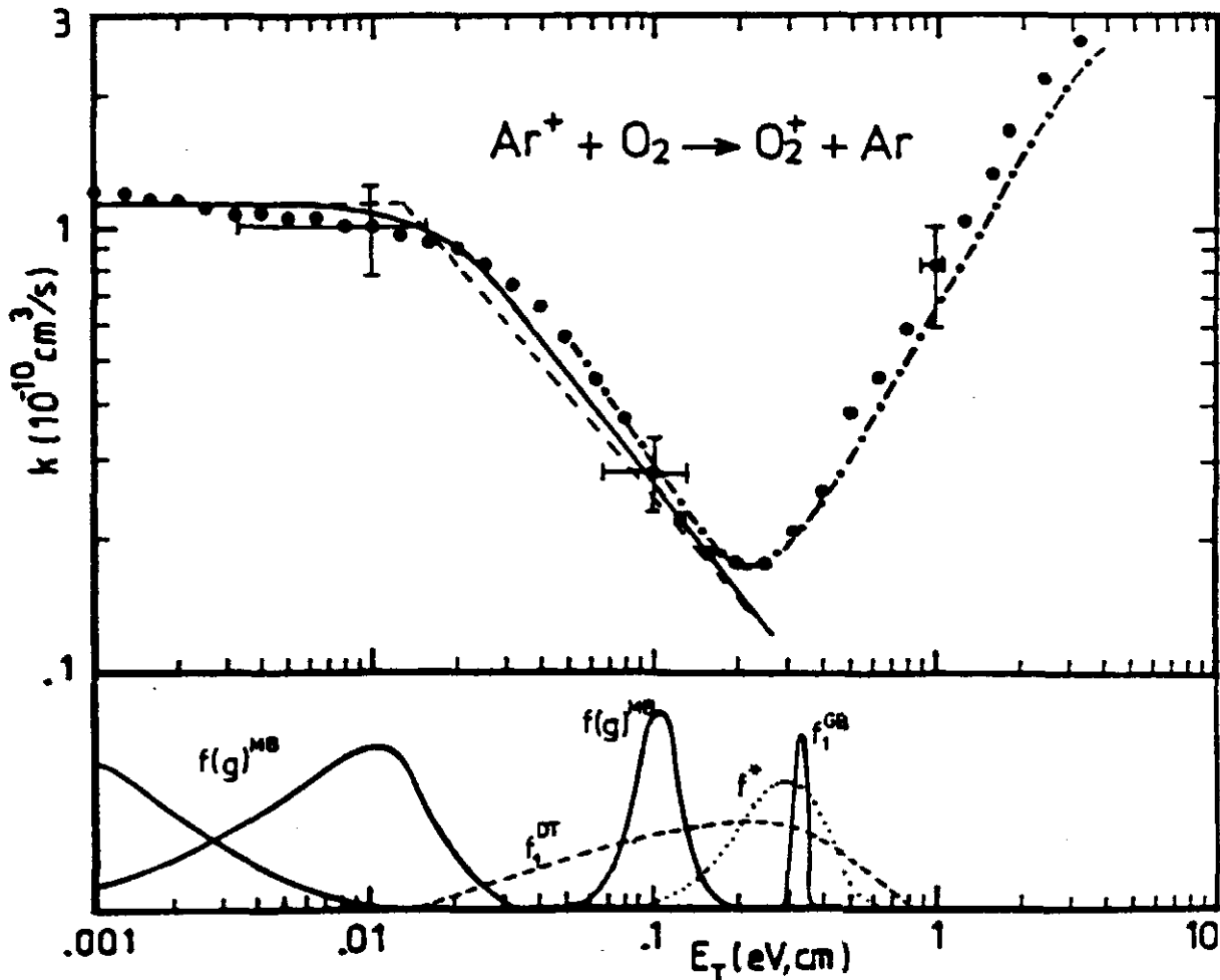
Figure 63. Integral cross section for the reaction \text{Ar}^+ + \text{O}_2 \rightarrow \text{O}_2^+ + \text{Ar} , measured with the merged beam (●) and the guided-ion-beam (●-●) methods (Scherbarth and Gerlich, 1989). The results are plotted as rate coefficients to emphasize the change in slope below 20 meV. The increase above 0.2 eV is due to the formation of \text{O}_2^+(a^4\Pi_u) . The low-energy behavior of the cross section has been approximated by the expression given in Eq. (120) (dashed line). Evaluation of Eq. (93) results in the effective rate coefficient (solid line). The lower part shows distributions of the relative velocity f(g)^{\text{MB}} for the merged-beam conditions. For comparison the functions f_1^{\text{GB}} , f_1^{\text{DT}} , and f^* [see Eq. (94)] are given for the guided ion beam and DRIFT tube apparatuses.
