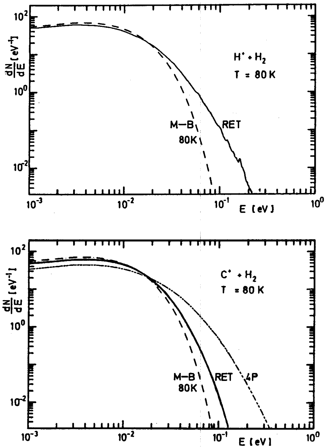
Figure 23. Log/log representation of numerically determined energy-distributions for H + (upper panel) and C + (lower panel) stored in a ring electrode trap (RET) with 80 K H 2 buffer gas. The comparison with the 80 K thermal Maxwell-Boltzmann (M-B) and the quadrupole trap (4P) distributions is discussed in the text.
