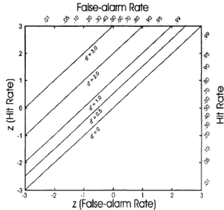
FIG. 1.2. ROCs for SDT on z coordinates.
