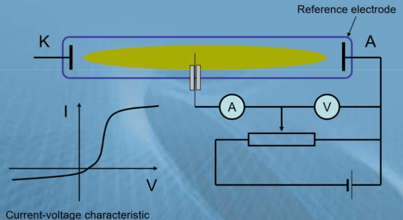
Current-voltage characteristic
