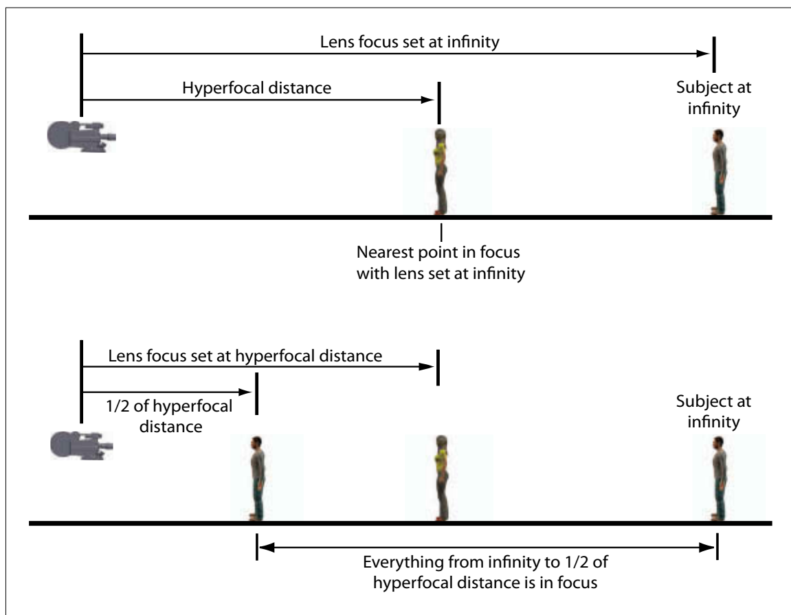
Figure 14.10. Two aspects of hyperfocal distance.
