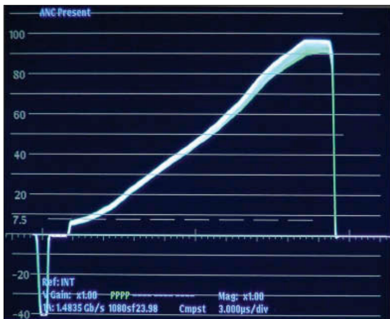
Figure 9.35. (top) Shot on the camera, this curve shows the gamma at normal, which is .45 on this camera.
