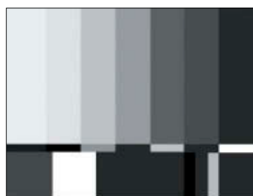
Figure 9.18. Incorrect luminance; notice how all three of the PLUGE bars in the lower right are visible.
