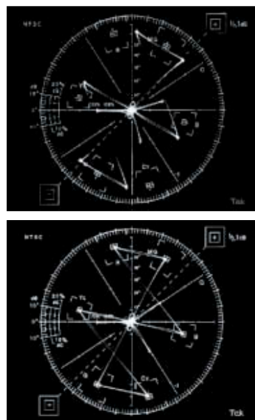
Figure 9.9. (top) Hue (phase) error ; notice how the color is shifted clockwise — the dots indicating the key hues are not in their proper boxes. (Photo courtesy of Tektronix.)
