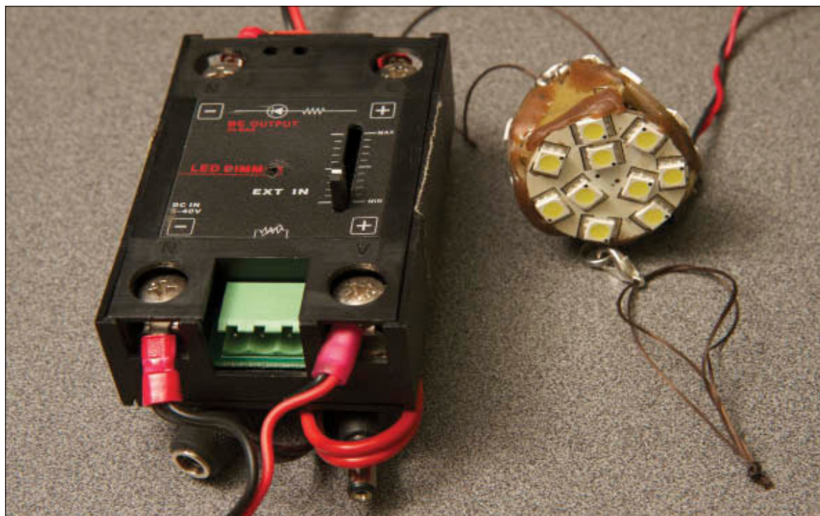
Figure 16.17. An on-the-set lighting effect (called a gag ) such as this will often be executed by the lighting department. This one, a glowing ball of light for The Sorcerer's Apprentice , was designed by Michael Gallart and executed by the legendary Billmo. It consists of a three-faced cluster of LEDs powered from a 12 volt DC source, run through an LED dimmer. It is shown in use in Figure 16.18.
