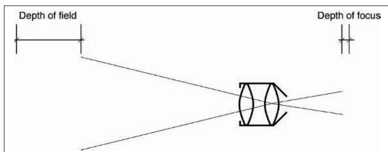
Figure 14.7 The difference between depth-of-field (in front of the lens, the subject) and depth-of-focus (behind the lens at the film plane).
