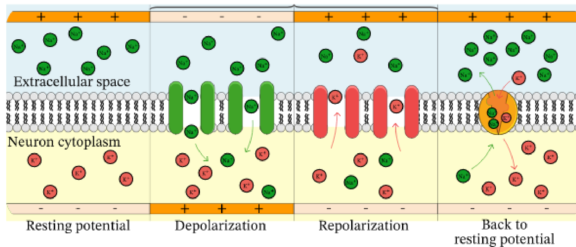
Action potential
