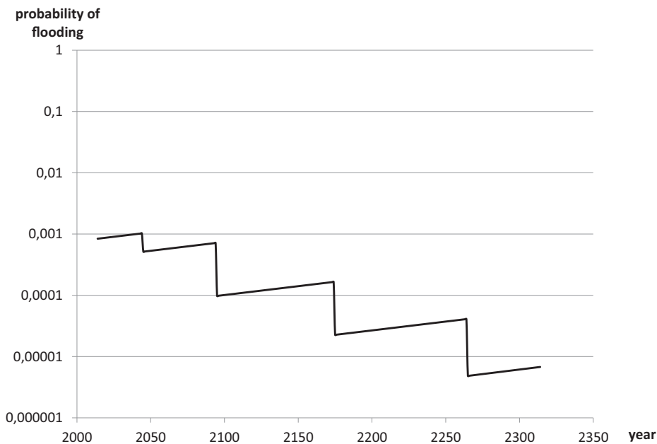
Fig. 1. Flood probabilities for dike ring 10 according to the optimal investment strategy, with the option of constructing anti piping measures only.
