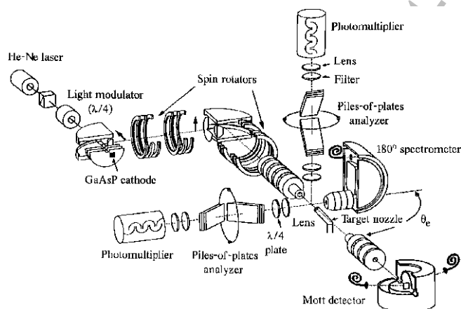
Figure 1: Experimental setup of Sohn and Hanne [2].
