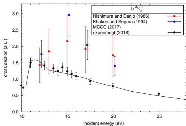
Figure 2: e-H 2 b 3 Σ u + excitation see Ref.[8] for details.
