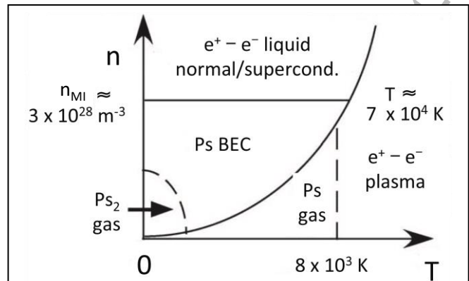
Fig. 1. Schematic (only) phase diagram of the electron-positron system as a function of density n and temperature T . The density n_{MI} of the metal-insulator transition is indicated. While this quantum phase is beyond current technology, \text{Ps}_2 has been created and studied, and near-term studies of a Ps BEC and a classical pair plasma are possible. For the future, more accurate calculations of key features of this phase diagram would be very useful.
