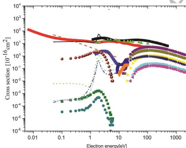
Figure 1; Summary of recommended cross section for electron collisions with the \text{NF}_3 molecule: Thick black line - total scattering, green triangle - elastic scattering, thick red line - momentum transfer, thin lines rotational excitation (red \Delta J=0 , black \Delta J=1 , green \Delta J=2 , dark blue \Delta J=3 , light blue \Delta J=4 ), brown circles, green squares and green circles – dissociative electron attachment, thick blue line – vibrational excitation, other symbols represent various combinations of ionisation and dissociation. For further details see Song et al [1].
