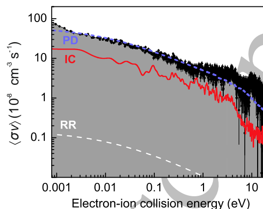
Figure 1 – Dielectronic recombination cross-section of W^{18+} ions ( 4f^{10} valence configuration) measured with the storage-ring merged-beams method. (Cross section \sigma multiplied with the collision velocity v and convolved with the electron energy spread.) Calculations show radiative recombination (RR), dielectronic recombination by one-electron promotion in intermediate coupling (IC), and a model including statistical partitioning and a damping correction (PD). (Adapted from Ref. [3]. Beam-merging artefacts at <0.001 eV are negligible in the plasma rate constants.)
