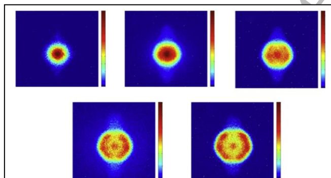
Figure 2. Velocity Map images of O - /OH - in acetaldehyde CH 3 CHO recorded at 9.0, 9.5, 10.0 10.5 and 11.0 eV showing two overlapping resonances distinguished by change in angular distributions [9].
