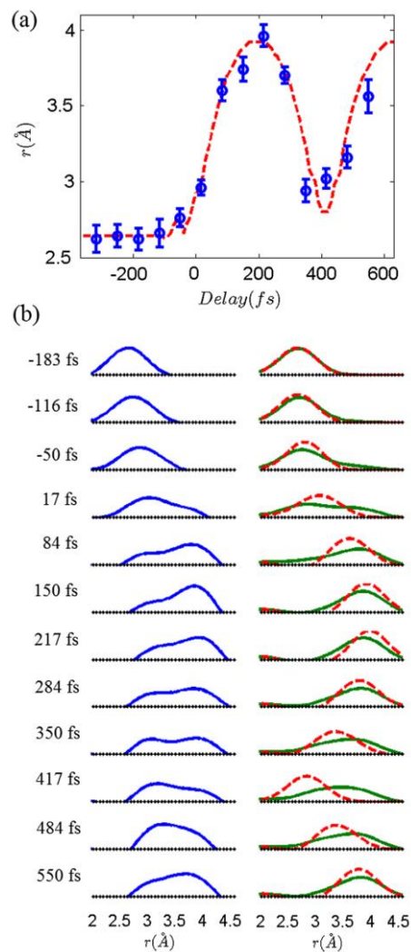
Figure 1. (a) Time-resolved experimental (blue circles with error bars) and simulated (red dashed line) bond lengths retrieved from the UED data. (b) The experimental (left panel) and simulated (right panel) time-resolved probability density function of the retrieved nuclear wave packet. The dashed red lines are the results of the theoretical calculations with the same spatial resolution as the experiment, and the solid green lines include also averaging due to the temporal resolution (230 fs). The black dotted line indicates the baseline for each curve. Reproduced from Ref.[6].
