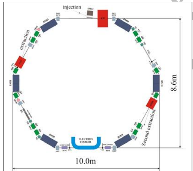
Figure 1 – A schematic drawing of ELENA under commissioning. Pulsed 5.3 MeV \bar{p} s from the AD are injected from the upper part (“injection”), cooled by the electron cooler and decelerated down to 100 keV, and finally transported to each experiment.
