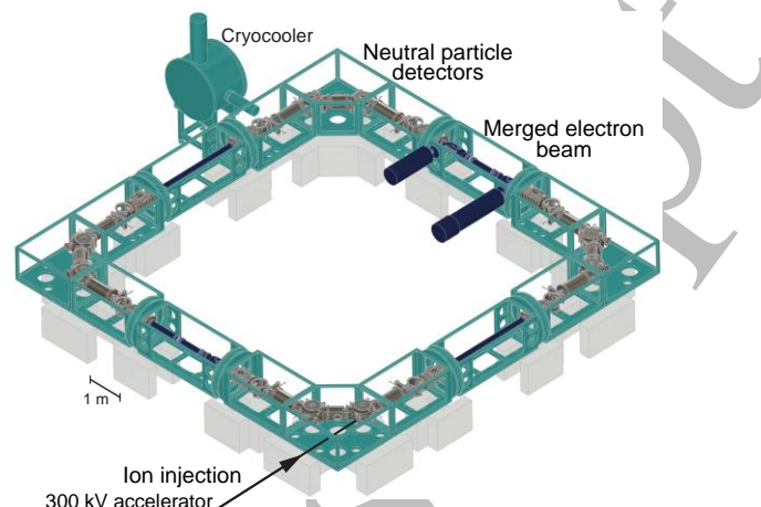
Figure 2 – The cryogenic electrostatic storage ring CSR that started operation in 2015 with the recently added electron beam section. The elements enclosing and steering the ion beam, the electron collision region and the particle detectors are operated below 10 K. (Adapted from Ref. [6].)
