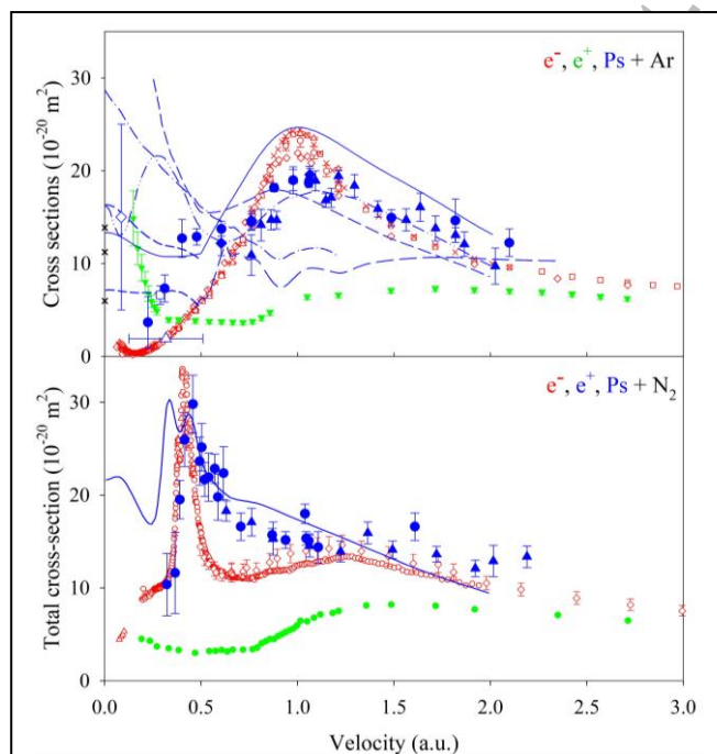
Figure 1 – Electron (red), positron (green) and Ps (blue) scattering from Ar and N_2 . Data points: experiments. Lines: Ps theories. For Ps: (solid symbols) total cross-section; (hollow symbols) momentum transfer cross-section. References in [7-10].
