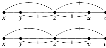
FIGURE 25. The definition of equidistance in terms of Pieri's relation.
