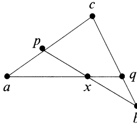
FIGURE 3. Inner Pasch Axiom.
