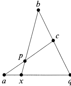
FIGURE 4. Outer Pasch Axiom.
