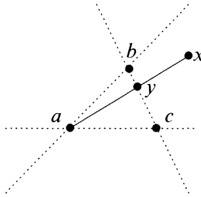
FIGURE 8. Alternative Form of Axiom 9 (2) .
