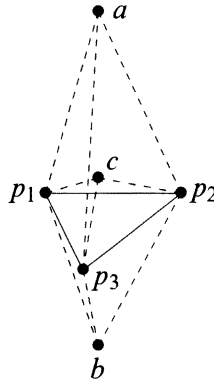
FIGURE 7. Upper 3-Dimensional Axiom.
